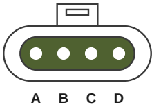
Harness plug – mating face
