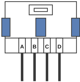
Harness plug – wire side
